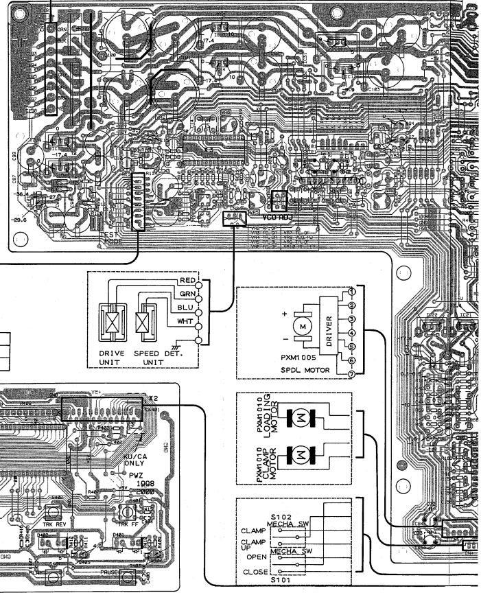
MAIN BOARD ASSEMBLY (PWZ1983:KU/CA TYPE) (PWZ1994:HEM AND SD TYPES)
