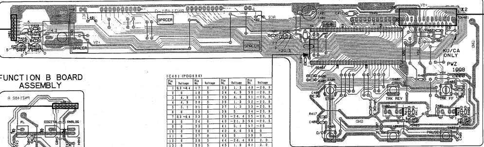
FUNCTION A BOARD ASSEMBLY (PWZ2000:KU/CA TYPE) (PWZ1998:HEM AND SD TYPES)
